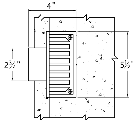
DRAIN DETAIL
